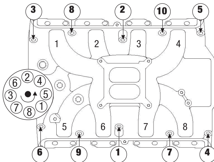
Figure 1 - 326-428 FE Ford Torque Sequence Torque Bolts to 25 ft/lbs. Firing Order: 1-5-4-2-6-3-7-8 Turn Distributor Clockwise to Advance Ignition Timing
