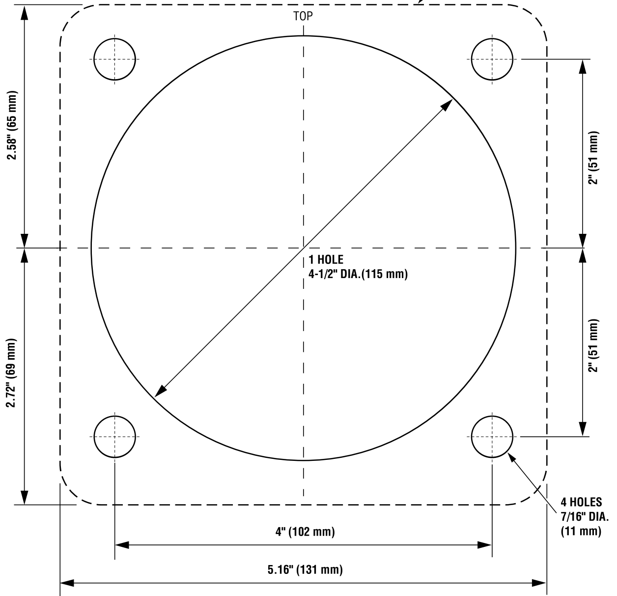
Figure 1. Mounting template.
